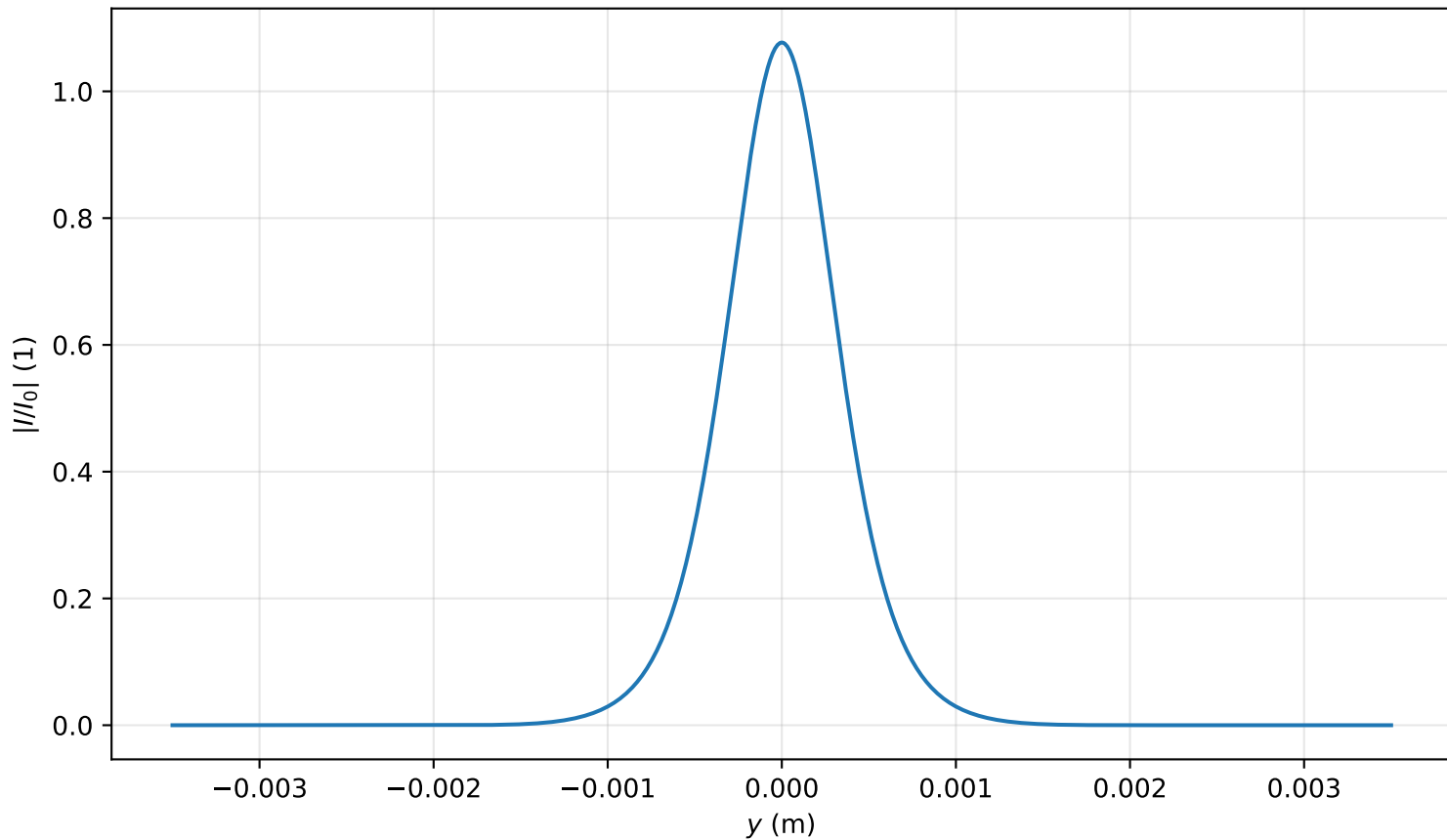
Intensity profile I(x = 0, y, z = 1.433)/I_0 , \text{Pin}=0.6\text{Pcr} , artificial time
